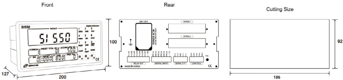
Physical Dimension [Unit:mm]
